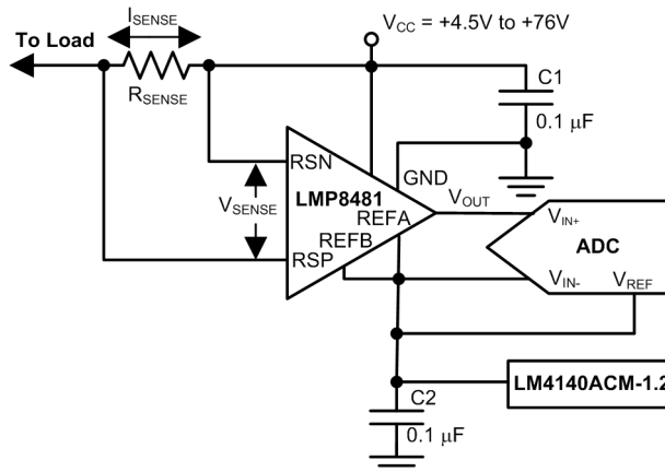
Figure 29. Bidirectional Current Sensing Using LMP8481
